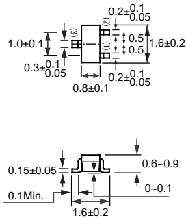
SC-75/SOT-416
