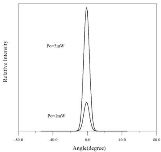
Far-Field Pattern(Parallel) vs. Optical Output
