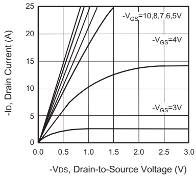
Figure 1. Output Characteristics
