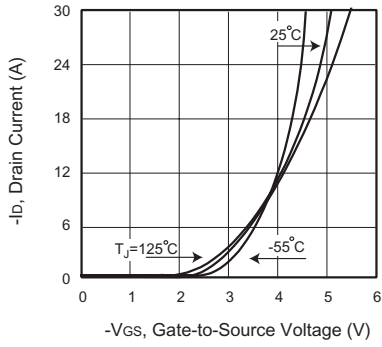
Figure 2. Transfer Characteristics
