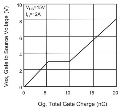
Figure 3. Gate Charge
