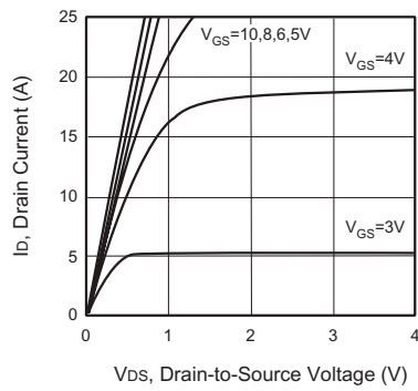
Figure 1. Output Characteristics
