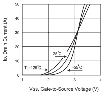
Figure 2. Transfer Characteristics
