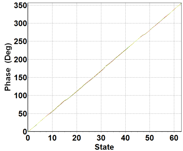
Peak phase (deg) versus Phase state Frequency = [5 – 6GHz], one chip
