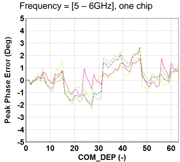
Peak phase error (deg) versus Phase State Frequency = [5 – 6GHz], one chip
