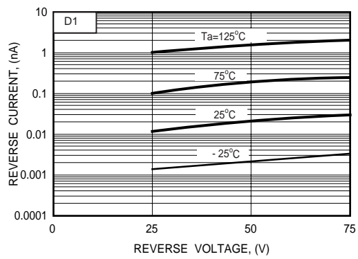
FIG. 3 - REVERSE CHARACTERISTICS
