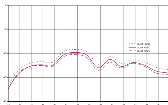
Conversion Loss, Image suppression UP Conversion – Infra-dyne mode - IF = 1.2GHz
