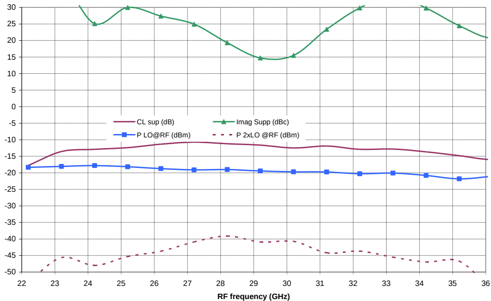
Conversion Loss, Image suppression & LO rejection UP Conversion - Supra-dyne mode - IF =1.2GHz
