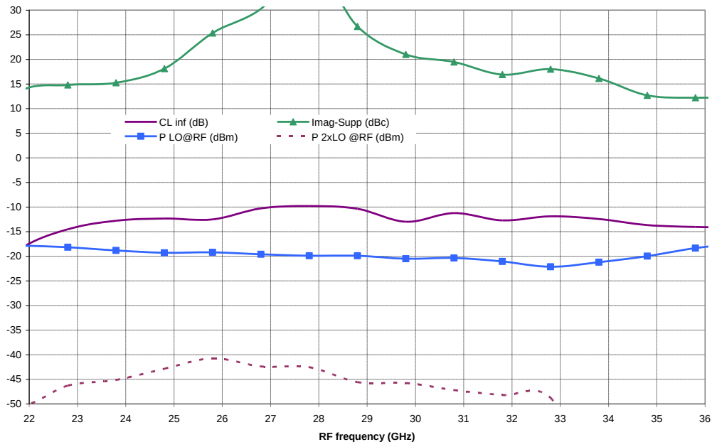
Conversion Loss, Image suppression & LO rejection UP Conversion - Infra-dyne mode - IF =1.2GHz
