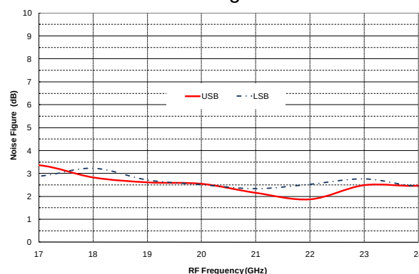
Noise figure
