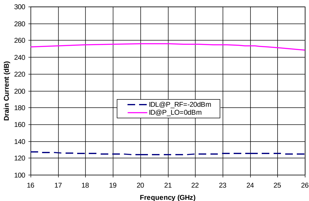
Figure 4: Drain Currents versus Frequency F_{RF} = 2 \times F_{LO} - F_{IF} , \text{Freq}_{IF} = 2.0\text{GHz} , GC2 = GC3 = -1.5\text{V}
