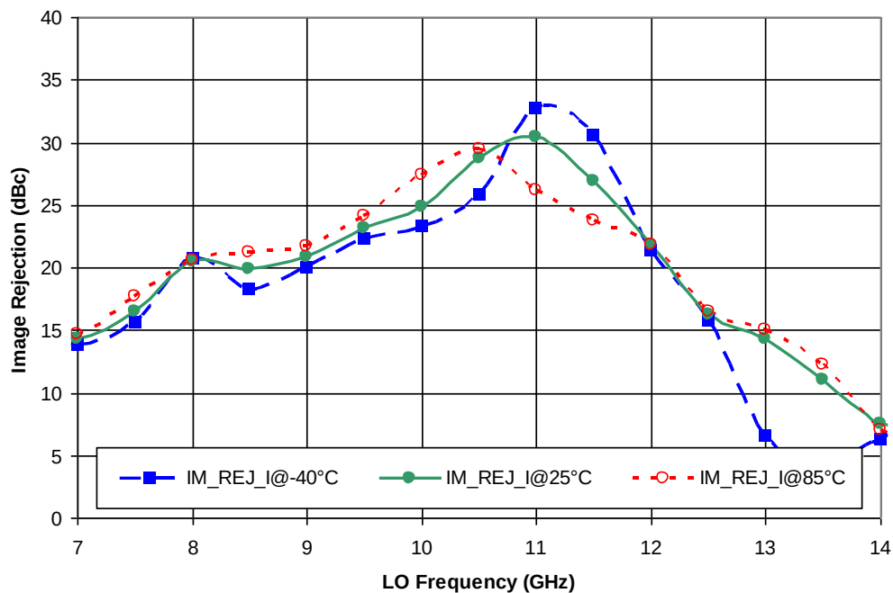
Figure 11: Image Rejection on Output I F IF = 2.0GHz, GC2 = GC3 = -1.5V
