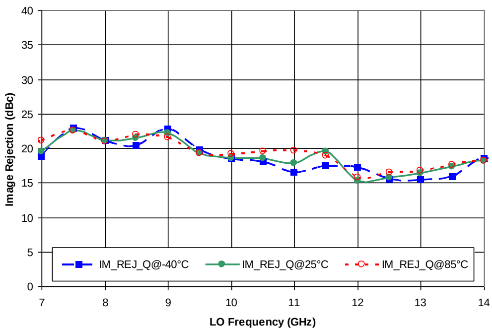
Figure 12: Image Rejection on Output Q F IF = 2.0GHz, GC2 = GC3 = -1.5V
