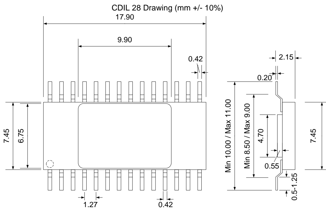
CSOIC 28 Drawing (mm +/- 10%)
