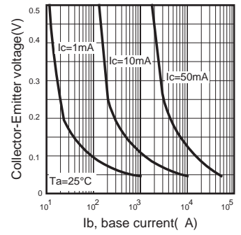
Fig.6 Collector saturation region
