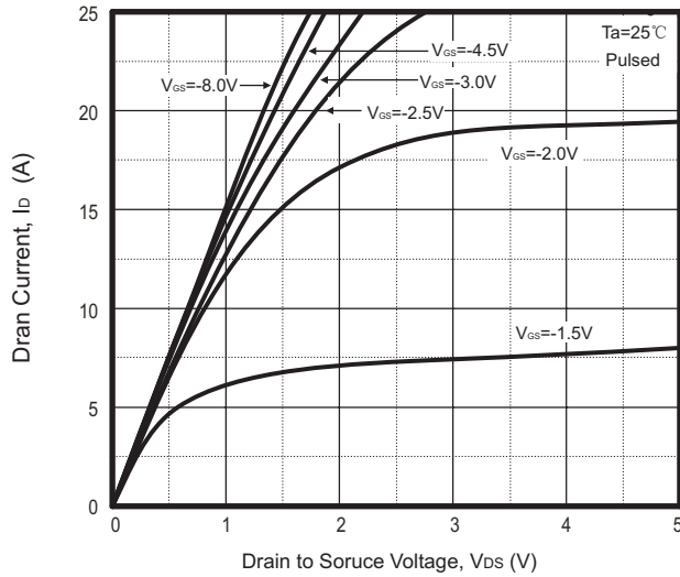
Fig.1 - Output Characteristics
