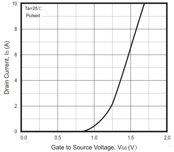
Fig.2 - Transfer Characteristics
