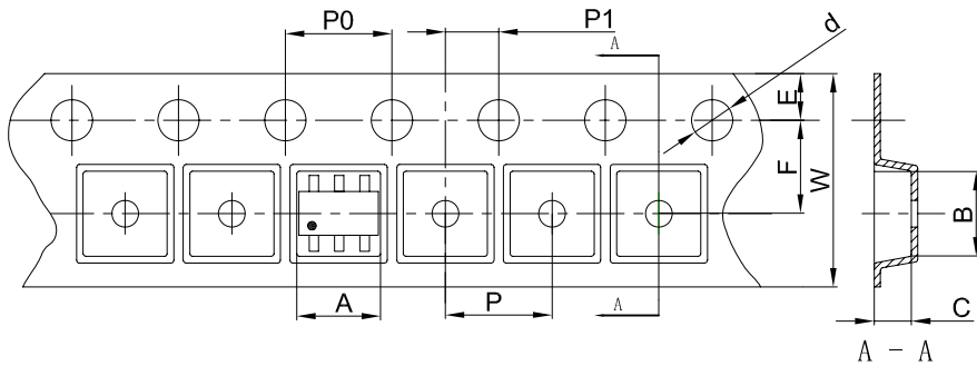
Dimensions are in millimeter
