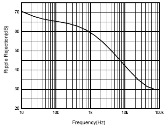
Figure 14. Ripple Rejection vs. Frequency
