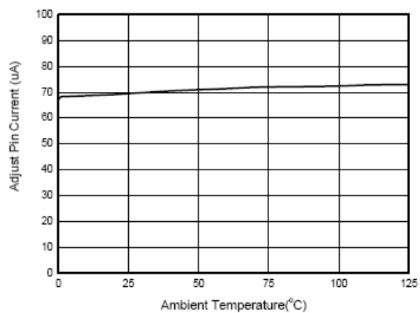
Figure 9. Adjust Pin Current vs. Temperature
