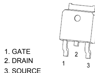
TO-252-2L
