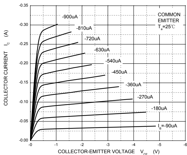
Static Characteristic
