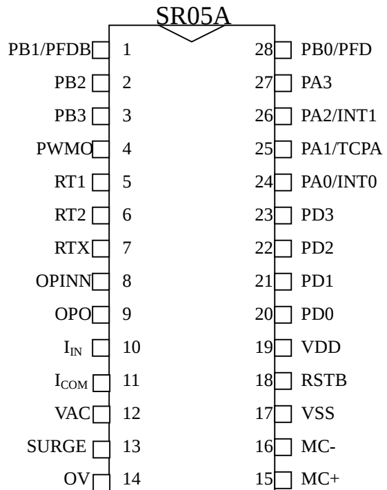
28-SDIP/DIP-A
