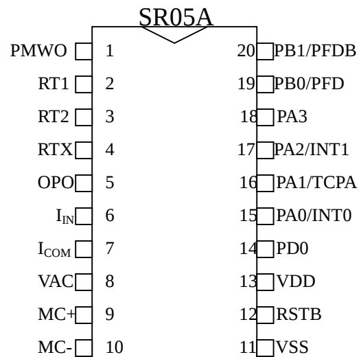
20-SDIP/DIP-C
