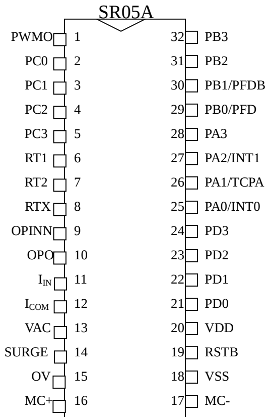
32-SDIP/DIP-A
