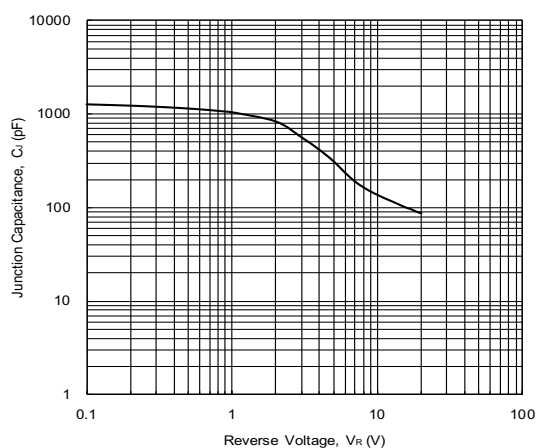
Fig. 5 - Junction Capacitance
