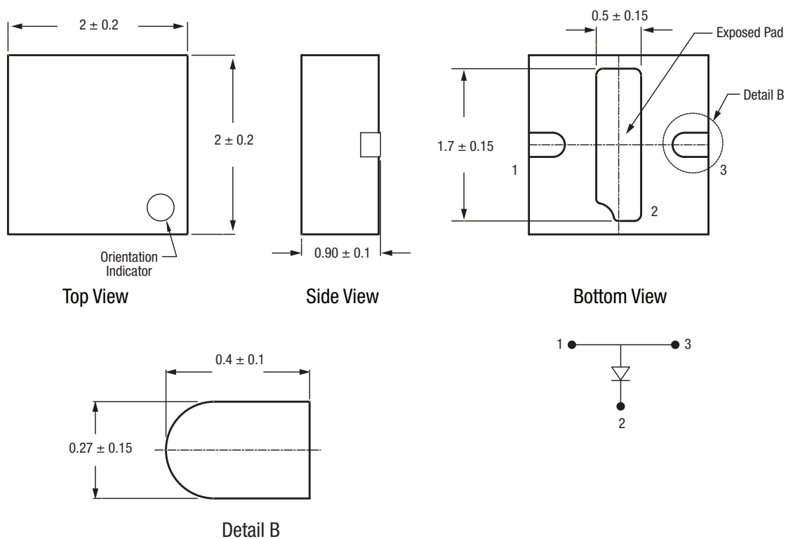
Figure 9. CLA4611-085LF QFN Package Dimension Drawing
