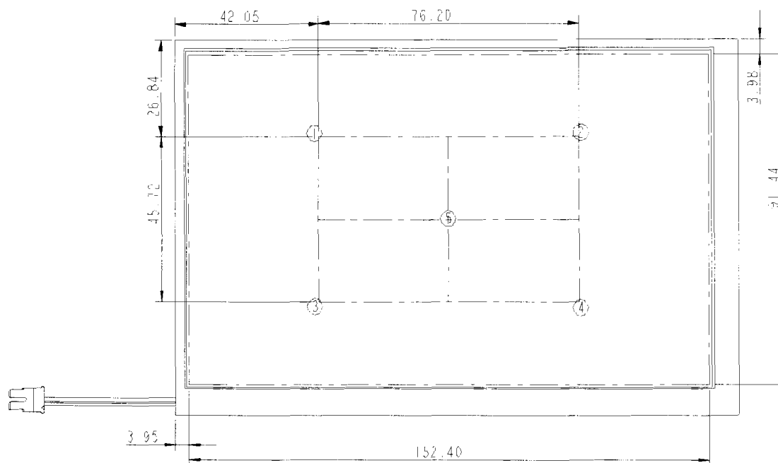
Fig.1 Measuring point
