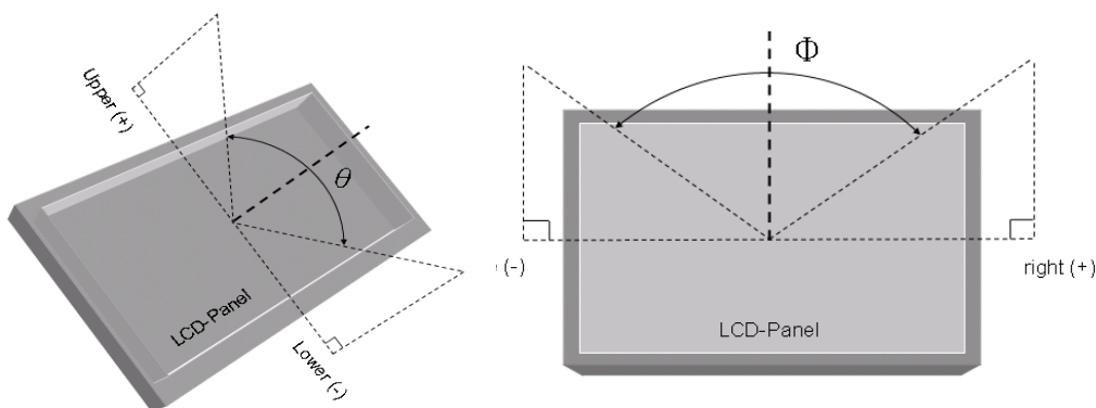
Fig.7-2 Definition of Viewing Angle
