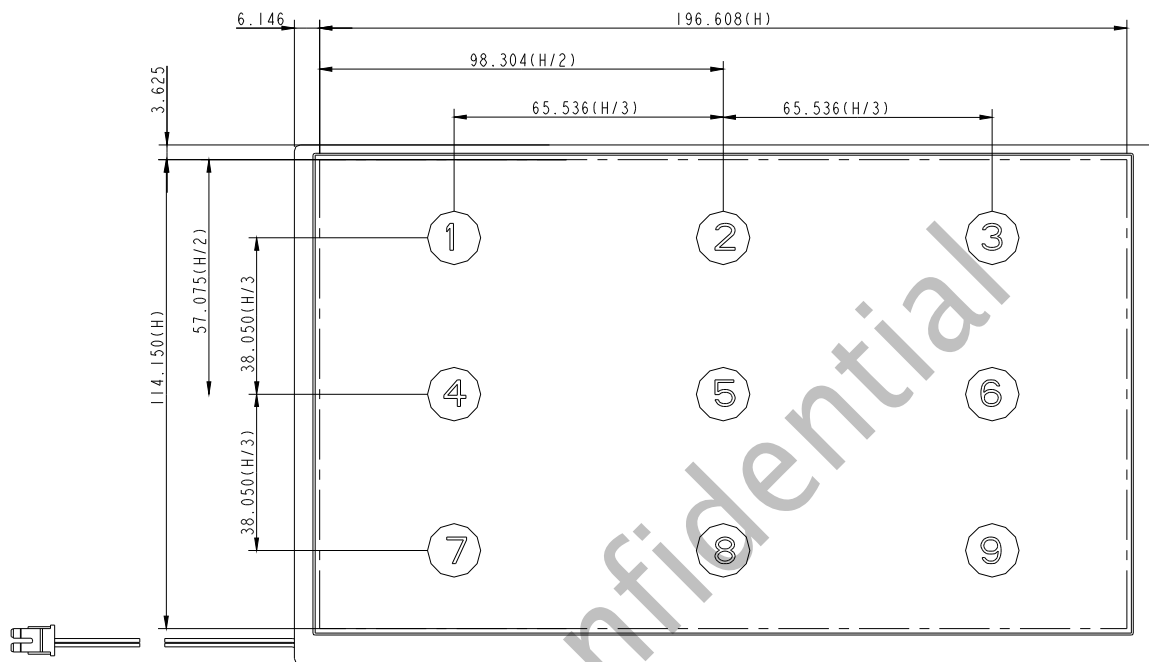
Fig.7-1 Measuring point
