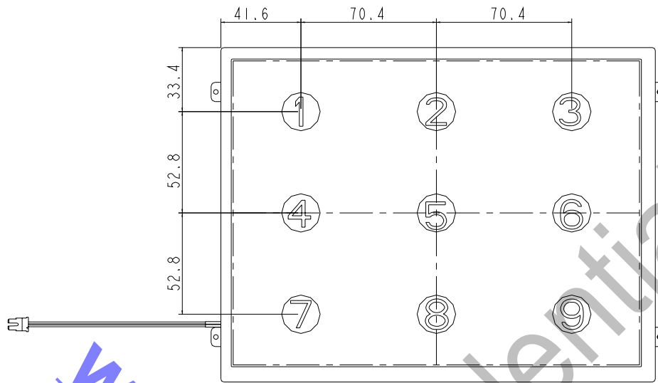
Fig8-1 Measuring point
