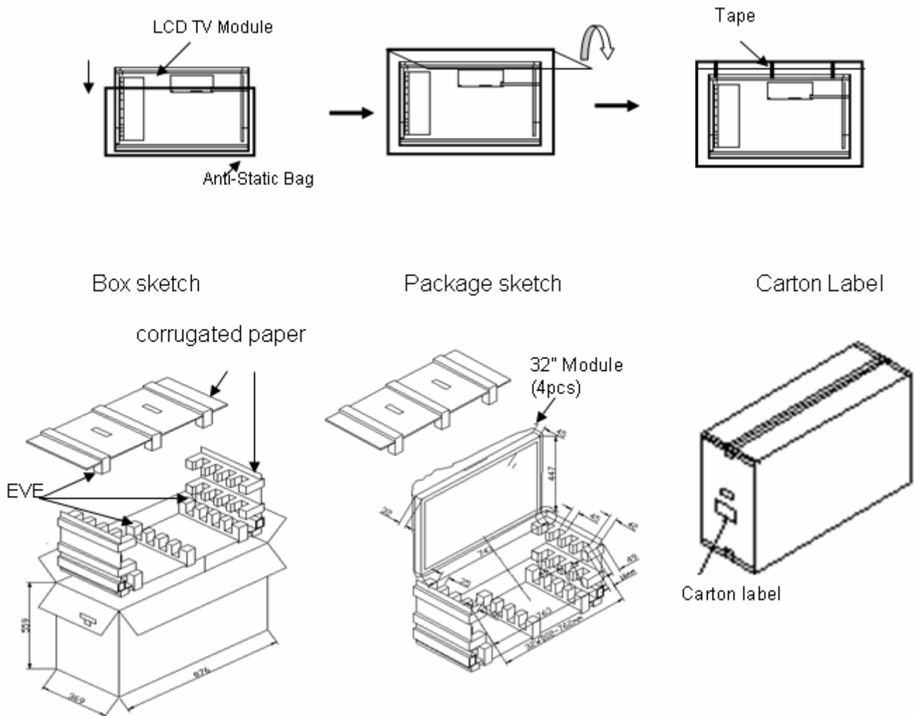
Figure 1 Packing Method
