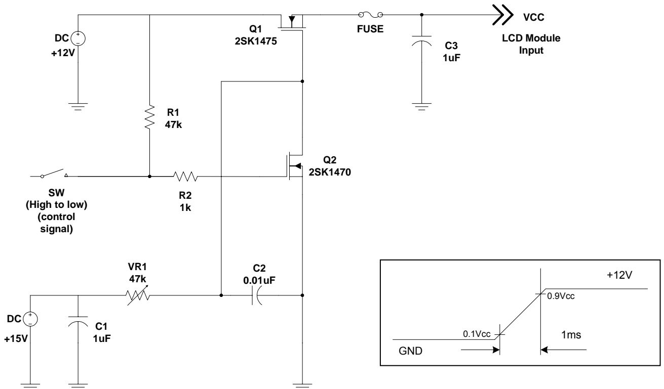
Vcc rising time is 1 ms
