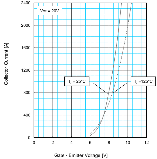
TRANSFER CHARACTERISTICS (TYPICAL)
