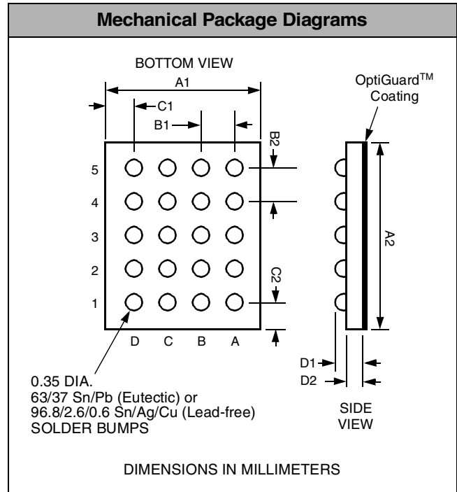
Package Dimensions for CM1205-16CS/CP 20-bump Chip Scale Package
