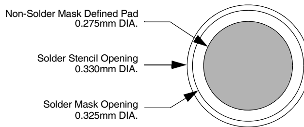
Figure 1. Recommended Non-Solder Mask Defined Pad Illustration
