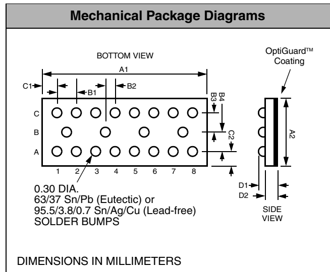
Package Dimensions for CM1405-03 Chip Scale Package
