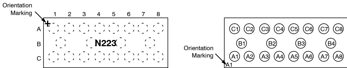
CM1422 CSP Package
