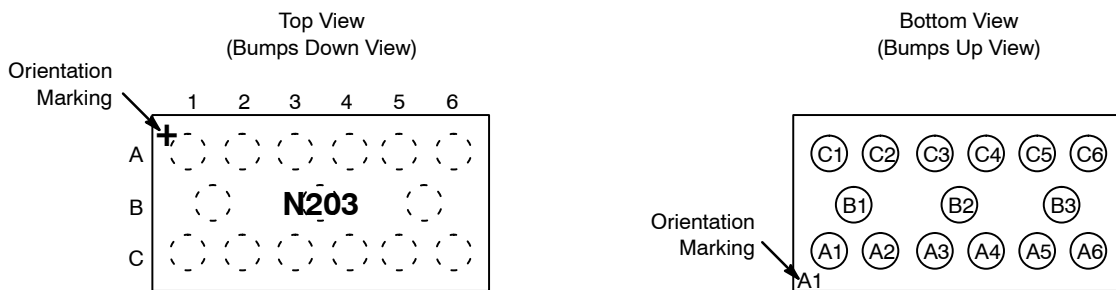
CM1420 CSP Package
