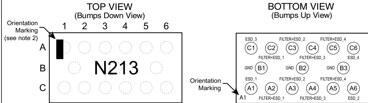
CM1421-03 CSP Package
