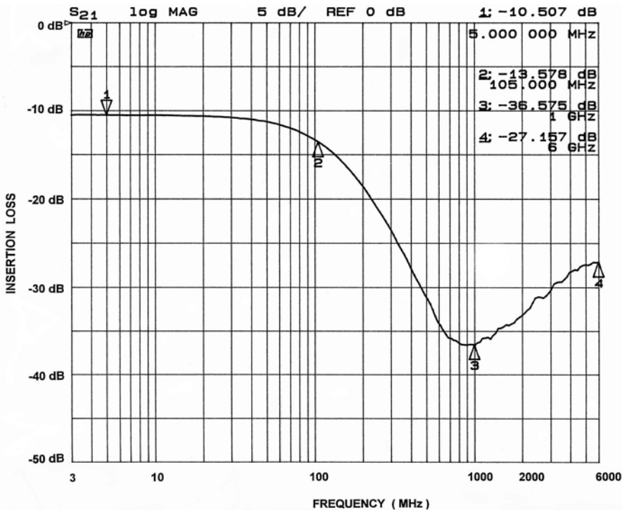
Figure 4. Channel 4 EMI Filter Performance (CM1436-04 only)
