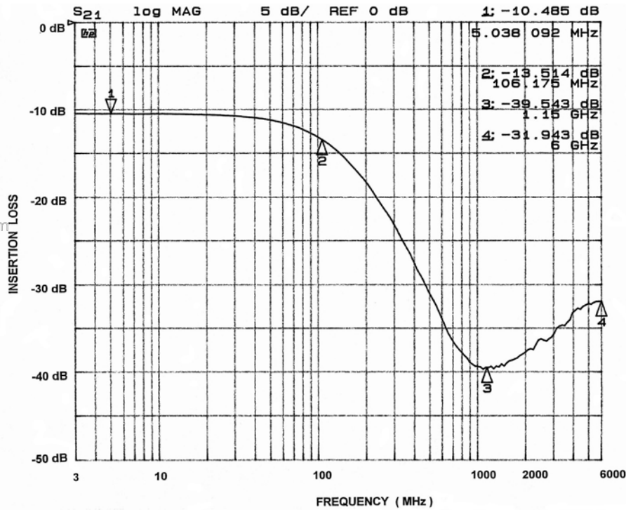
Figure 3. Channel 3 EMI Filter Performance (CM1436-04 only)
