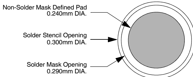
Figure 4. Recommended Non-Solder Mask Defined Pad Illustration
