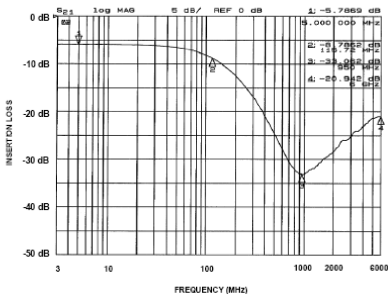
Figure 8. Insertion Loss vs. Frequency (FILTER8 Input to GND)
