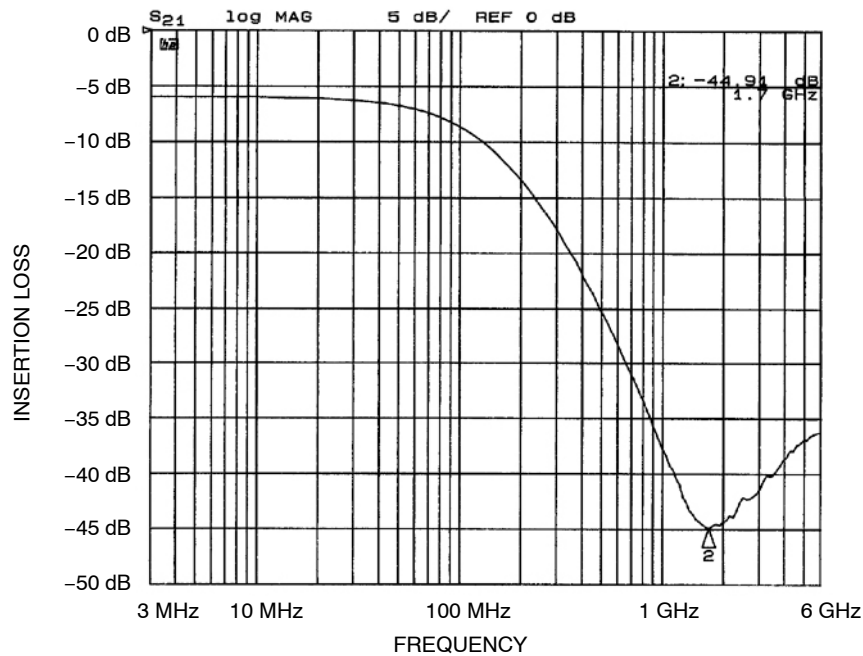
Figure 2. Insertion Loss vs. Frequency (FILTER2 Input to GND, CM1631-04DE)
