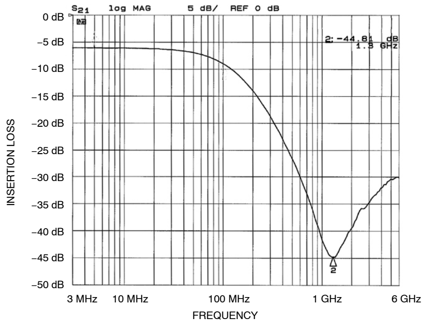
Figure 5. Insertion Loss vs. Frequency (FILTER1 Input to GND, CM1631-06DE)
