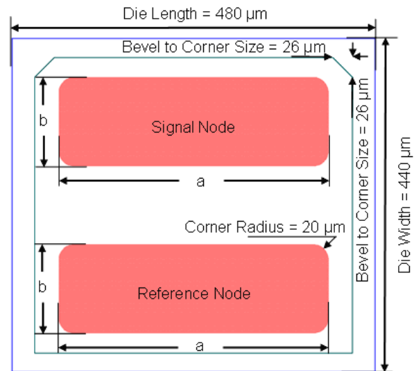
Package Dimensions
