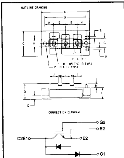
CM200E3Y-12E Outline Drawing
