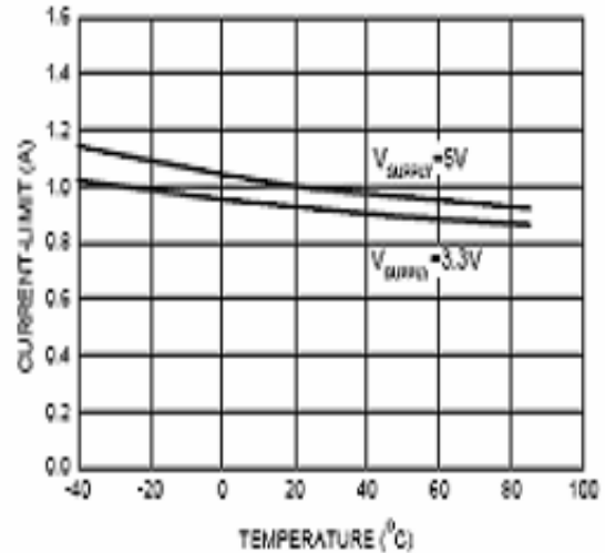
Short-Circuit Current-Limit vs. Temperature
