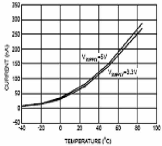
Off-Current vs. Temperature
