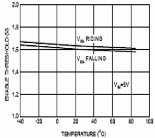
Enable Threshold vs. Temperature
