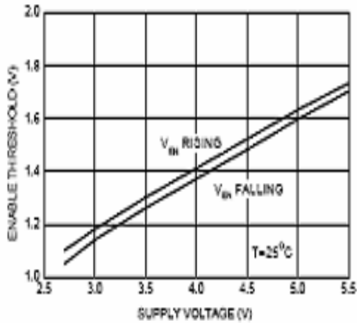
Enable Threshold vs. Supply Voltage
