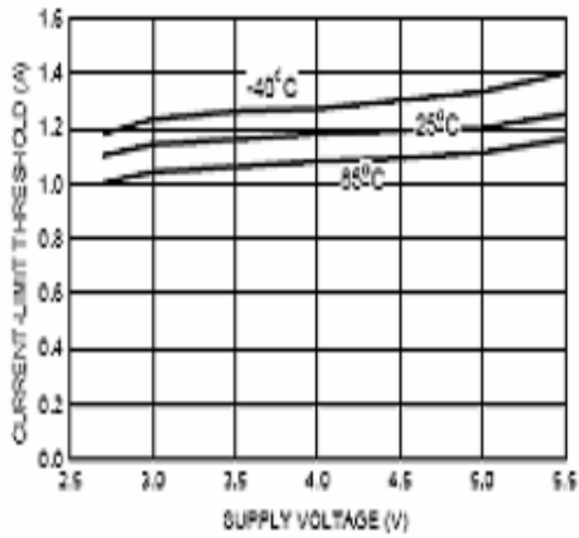
Current-Limit Threshold vs. Supply Voltage
