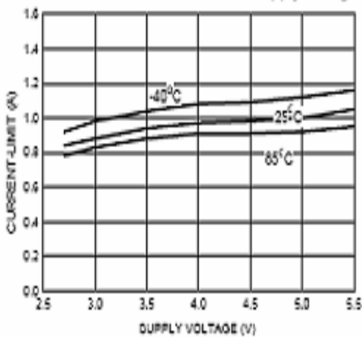
Short-Circuit Current-Limit vs. Supply Voltage
