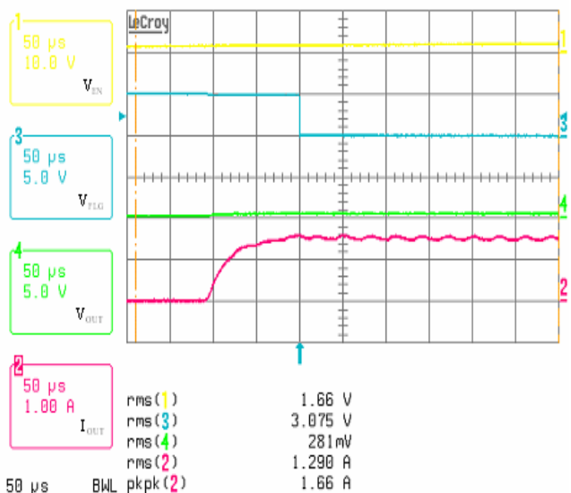
Current Limit
