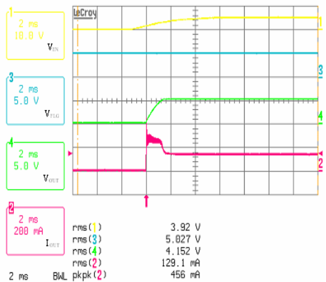
Enable Into Short
