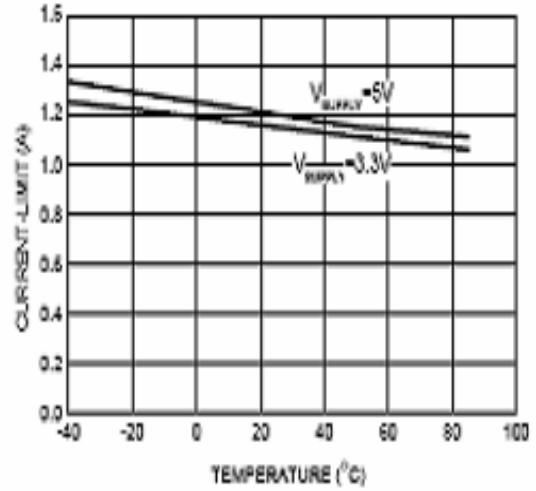
Current-Limit Threshold vs. Temperature
