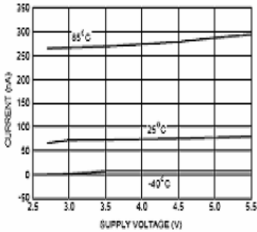
Off-Current vs. Supply Voltage
