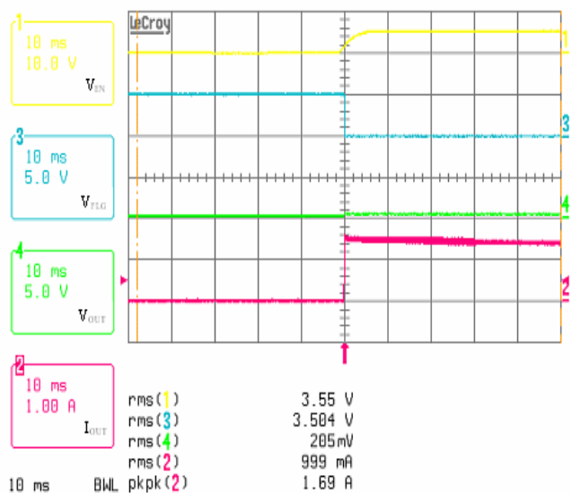
Current Limit
