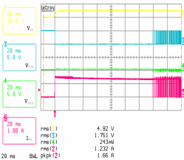
Current Limit
