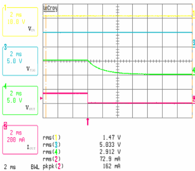
Current Limit
