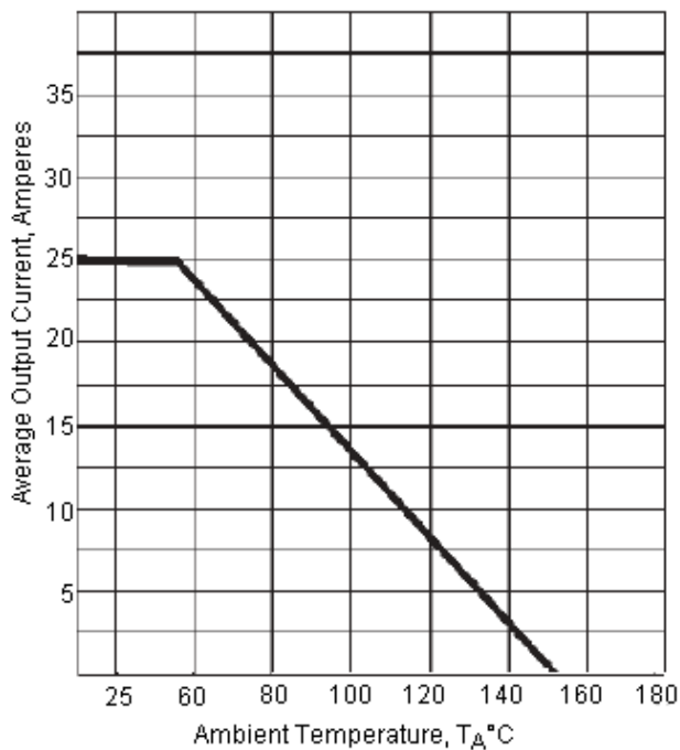
Output Current VS. Ambient Temperature Resistive or Inductive Load Bridge Mounted on 8 x 8 inches Aluminium Plate 25 inches Thick
