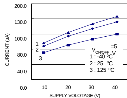
Shutdown Quiescent Current
