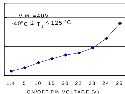
ON/OFF Pin Current (Sinking)
