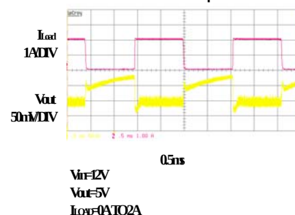
Load step
