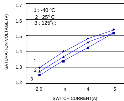
Switch Saturation Voltage
