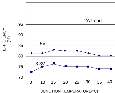
Efficiency
