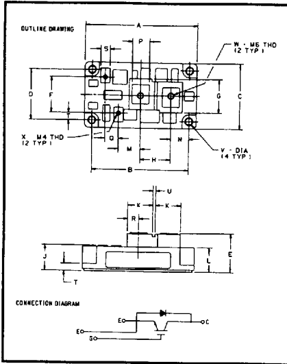
CM300HA-24E Outline Drawing
