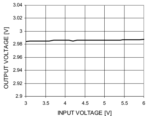
Figure 5. Line Regulation ( I_{LOAD}=5\text{mA} )
