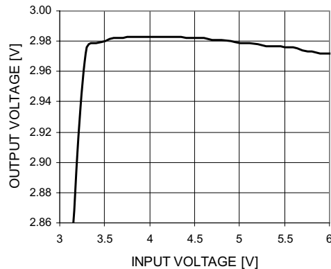
Figure 4. Line Regulation ( I_{LOAD}=300\text{mA} )
