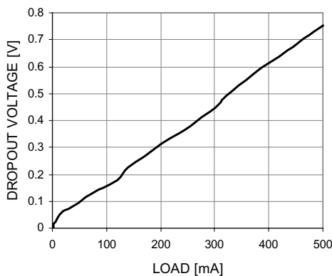
Figure 2. Dropout Voltage ( V_{OUT}=2.9\text{V} )
