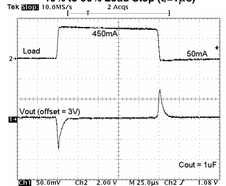
10% to 90% Load Step (t r =1µs)
