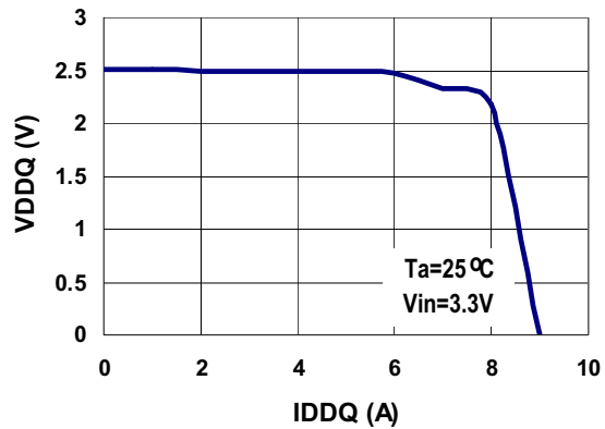
VDDQ vs. Load Current
