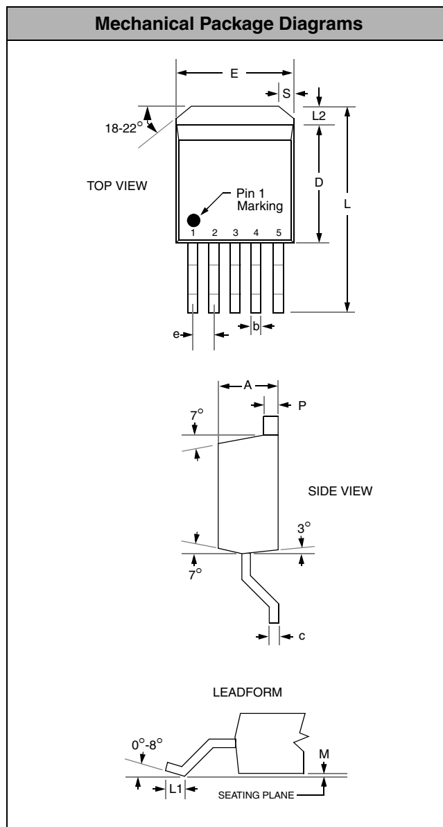
Package Dimensions for Standard TO-263
