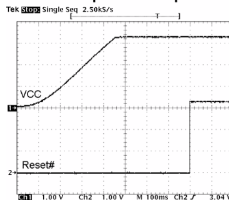
Power-up Reset Response
