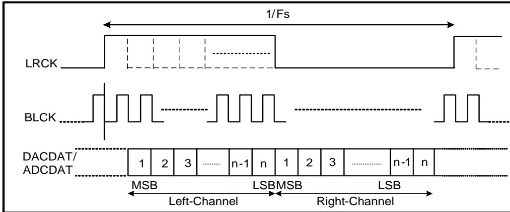
Figure 13. PCM Stereo Data Mode A Format (BCLK POLARITY=0)
