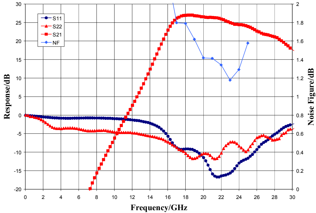
Broadband Performance, V_{dd} = 3.0\text{ V} , V_{gg} = 1.5\text{ V} , I_{dd} = 26\text{ mA} , T_A = 25\text{ }^\circ\text{C}
