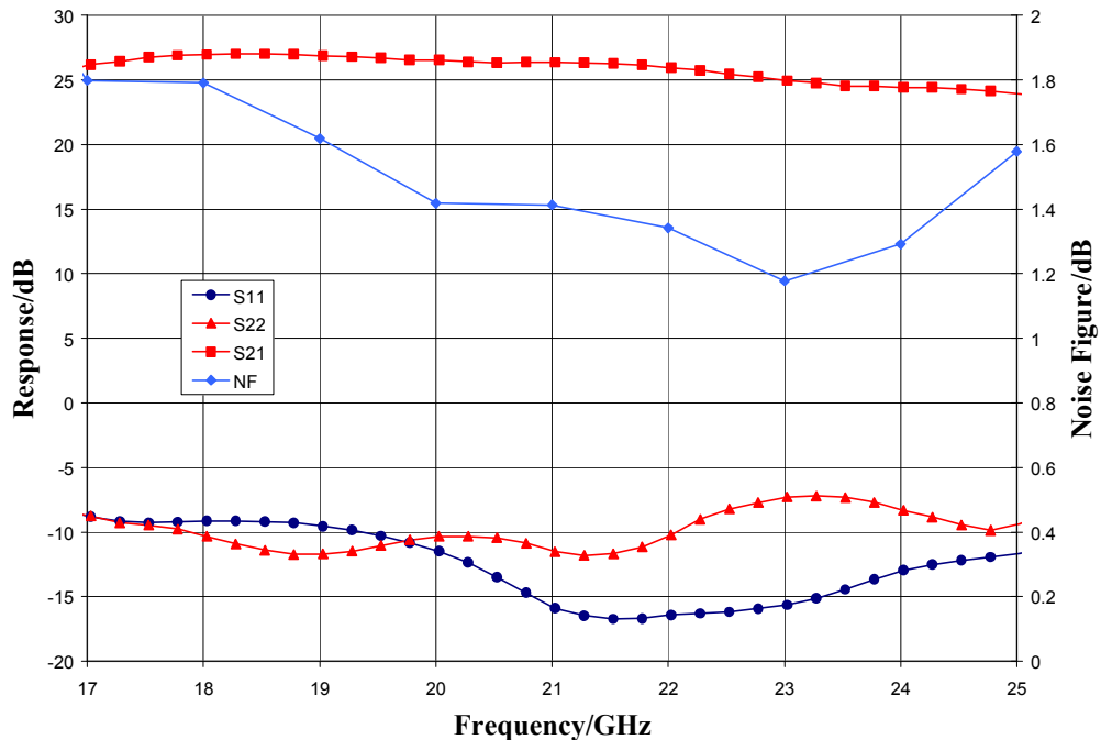
Narrow-band Performance, V_{dd} = 3.0\text{ V} , V_{gg} = 1.5\text{ V} , I_{dd} = 26\text{ mA} , T_A = 25\text{ }^\circ\text{C}
