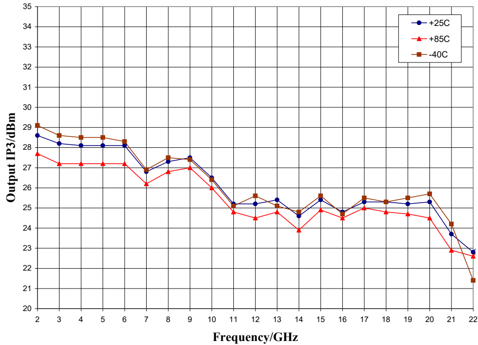
Output IP3 vs. Temperature, V_{dd} = 5\text{ V}
