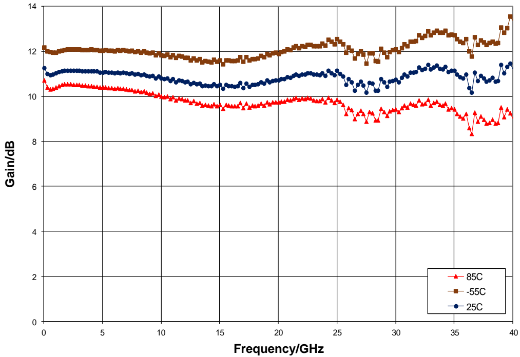
Gain vs. Temperature, V_{dd} = 8\text{ V} , V_{gg} = -0.32\text{ V}
