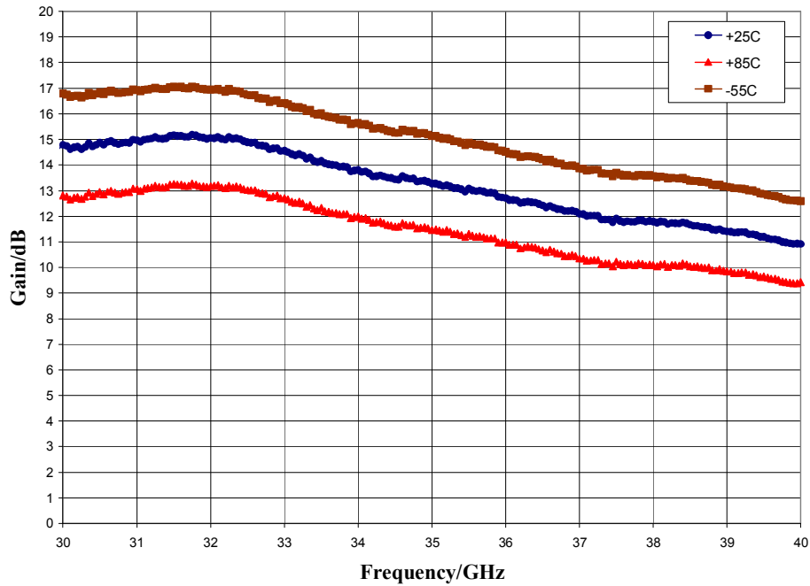
Gain vs. Temperature, V_{dd} = 3.0\text{ V} , V_{gg} = 3.0\text{ V}
