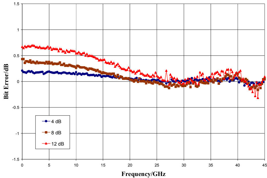
Bit Error versus Frequency, T_A = 25^\circ\text{C}
