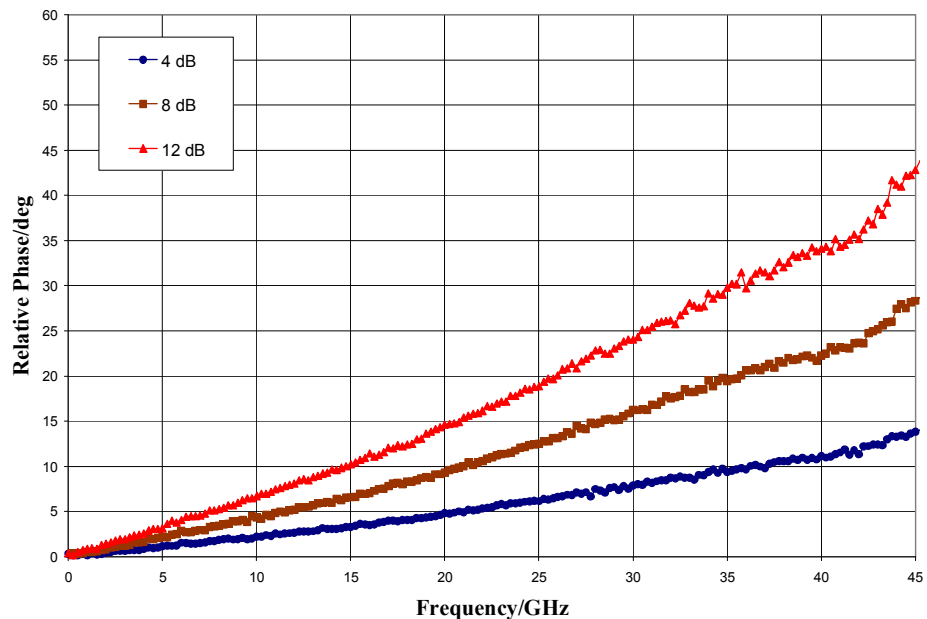
Relative Phase versus Frequency, T_A = 25^\circ\text{C}
